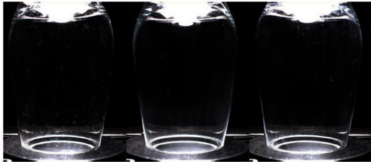
Standard alcohol alkoxylate
